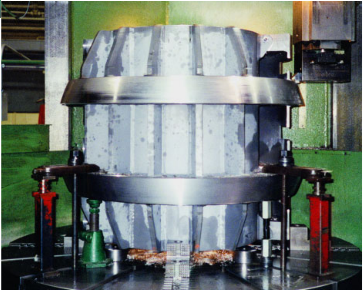
Main propulsion line shaft bearing for U.S. Navy vessel.
